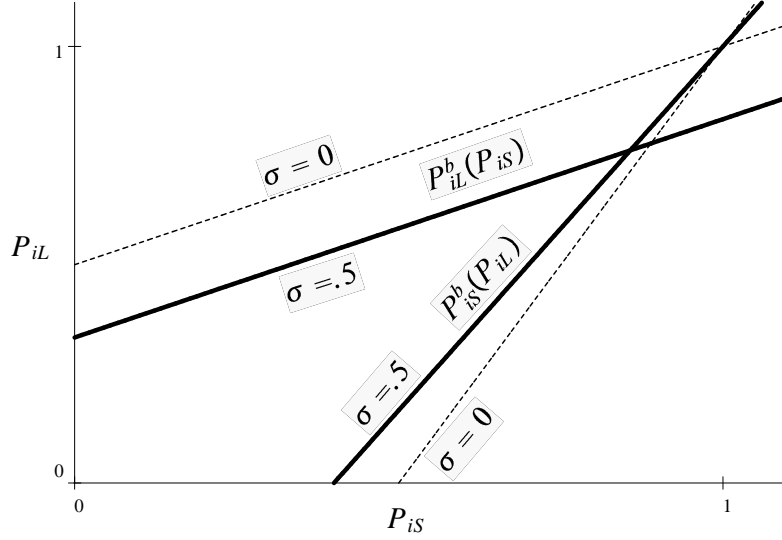
Figure 1: Best-response functions.
